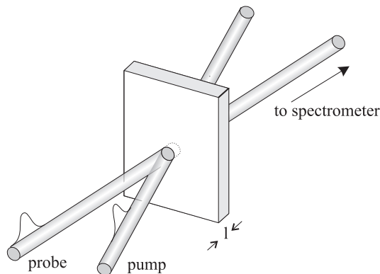
FIG. 8. Schematic representation of the pump-probe experiment. A sample of thickness l is illuminated by a pump pulse, which excites a significant fraction of the molecules. Next a time-delayed probe pulse is used to monitor the spectral changes induced by the first pulse.
